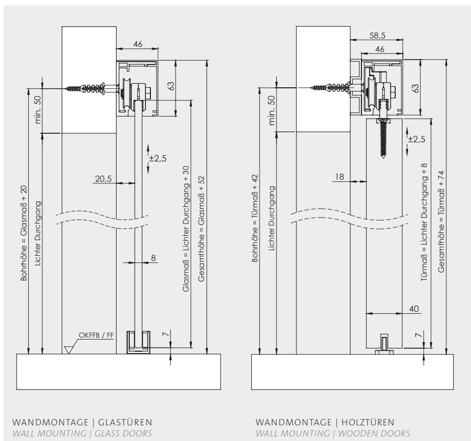
PLANEO 60 PRO WANDMONTAGE WALL MOUNTING
